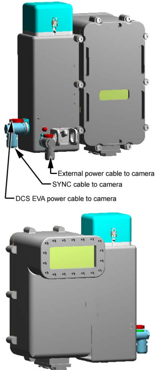
EVA Flash Mechanical Design
