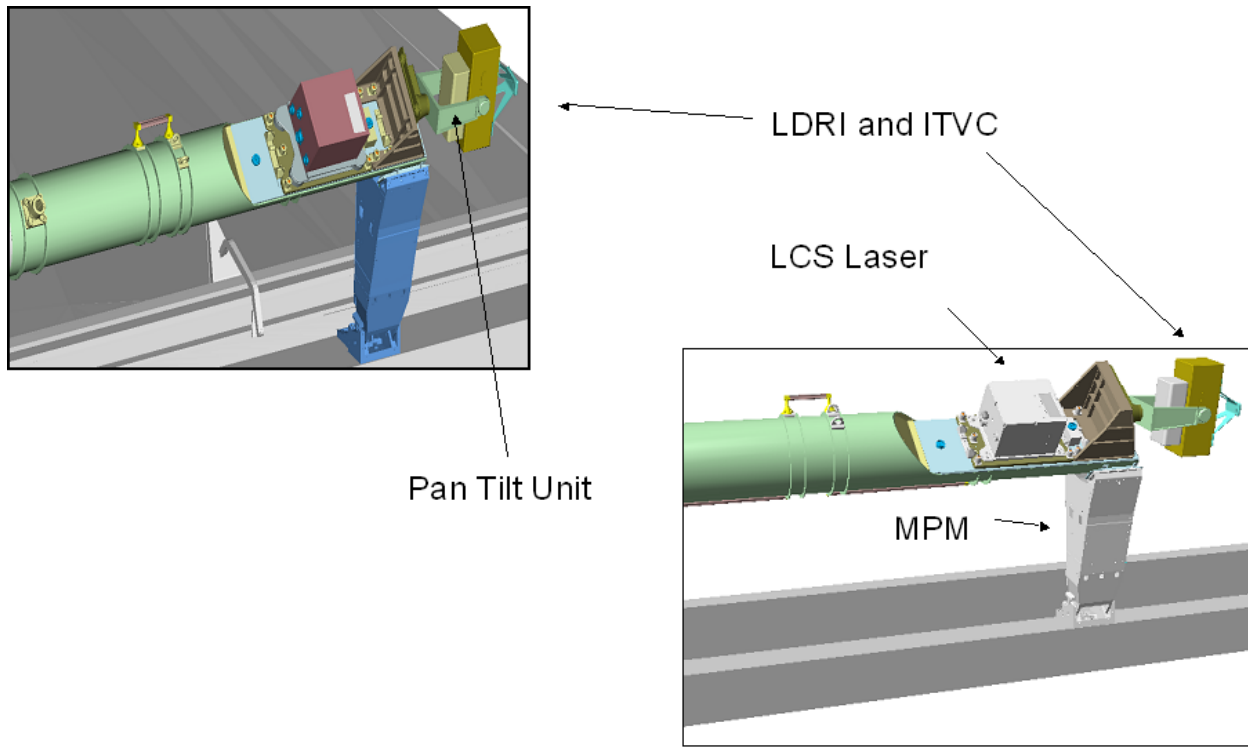
Inspection Sensors
